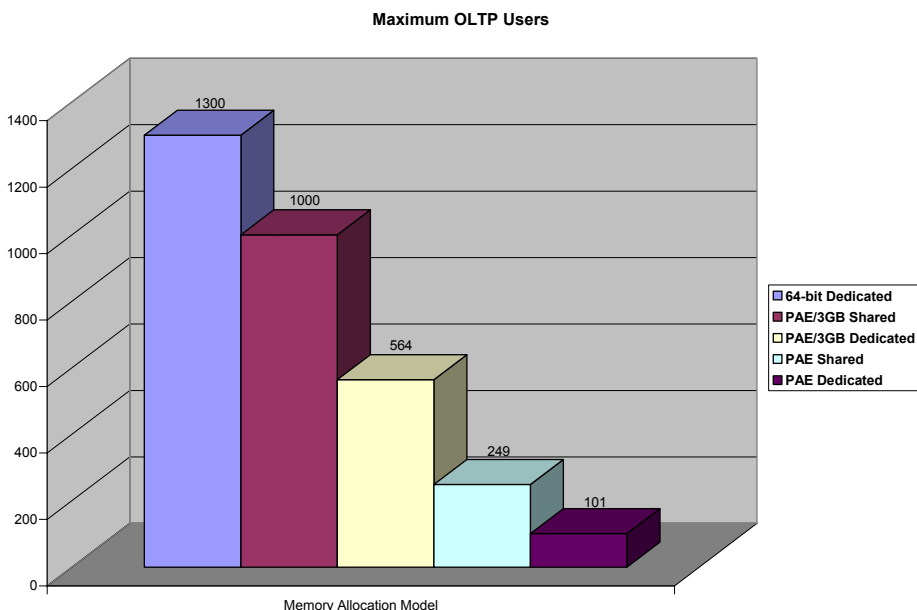
Figure 3 Maximum OLTP Users for each Memory Allocation Model
