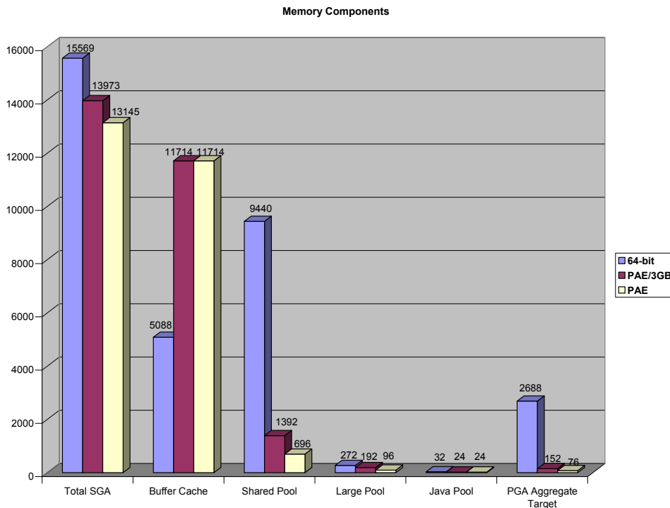
Figure 1 Memory Components of 32-bit and 64-bit Tests
