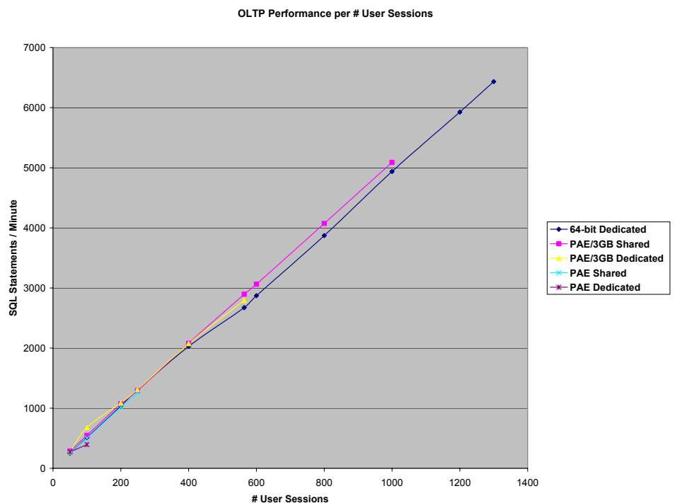
Figure 2 OLTP Performance per # User Sessions
